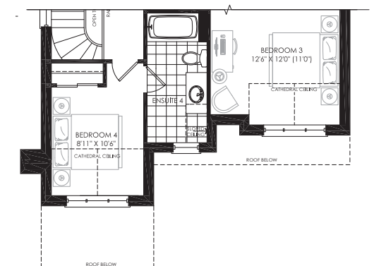
PARTIAL SECOND FLOOR PLAN ELEV. 'D'
