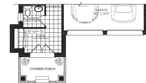
PARTIAL GROUND FLOOR PLAN ELEV. 'D'
