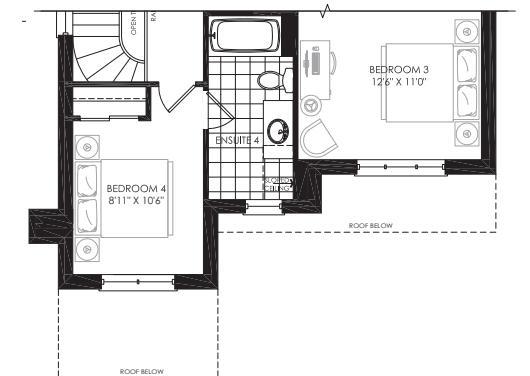
PARTIAL SECOND FLOOR PLAN ELEV. 'B'
