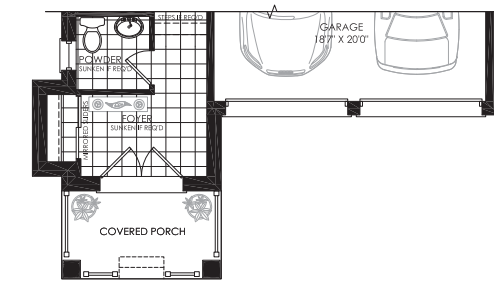
PARTIAL GROUND FLOOR PLAN ELEV. 'B'
